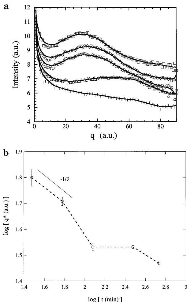
Figure 6. (a) Radial averages of 2D-FFT of the optical micrographs of Figure 5 at T = 180^\circ\text{C} . From bottom to top: t (min) = 30, 60, 120, 300, and 540. The peak position of each curve is denoted by q^* . (b) Variation of q^* with annealing time indicates initial conventional phase separation behavior, indicated by a t^{-1/3} behavior, but a plateau at later times is indicative of inhibited coalescence. At still longer times, the droplets coalesce, as shown in the AFM plots of Figure 8.
